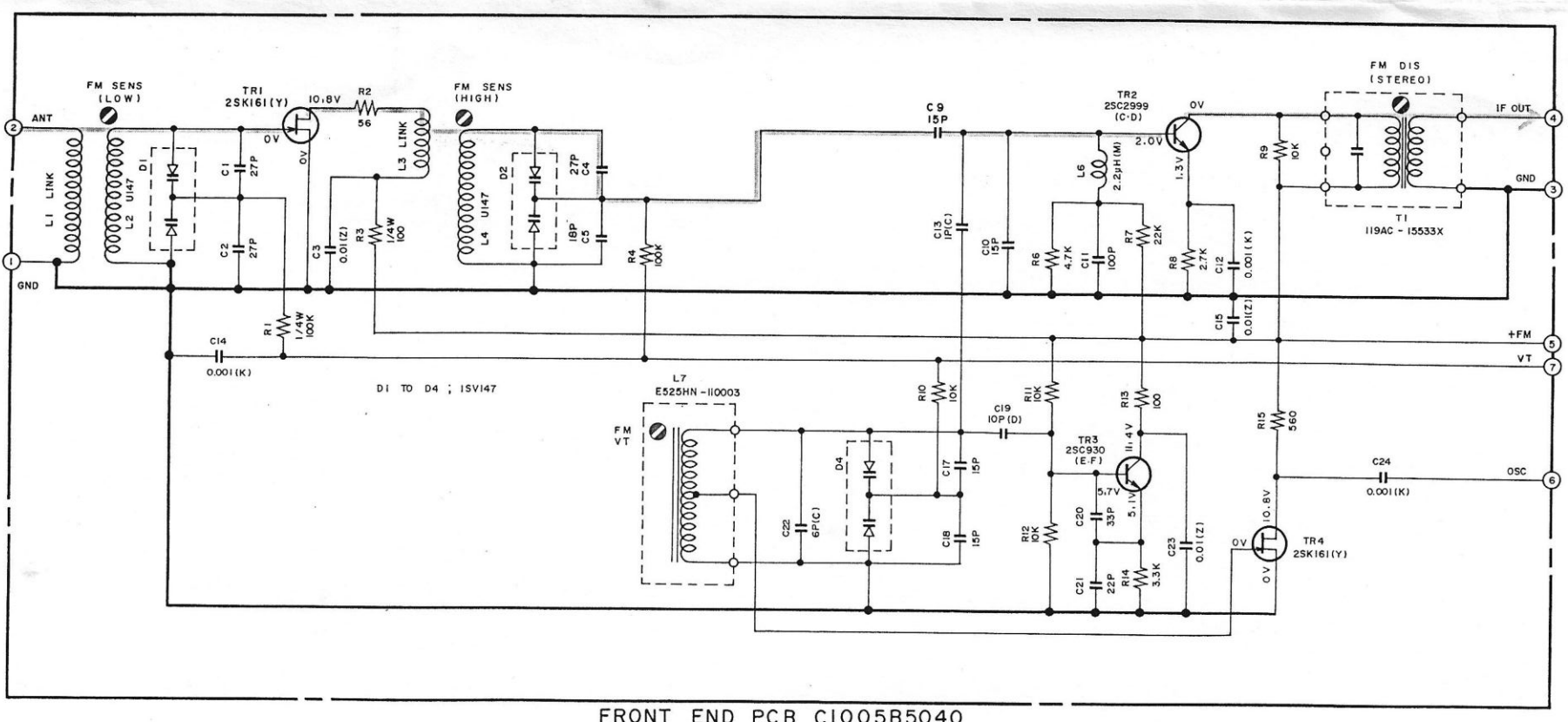
FRONT END PCB CI005B5040
