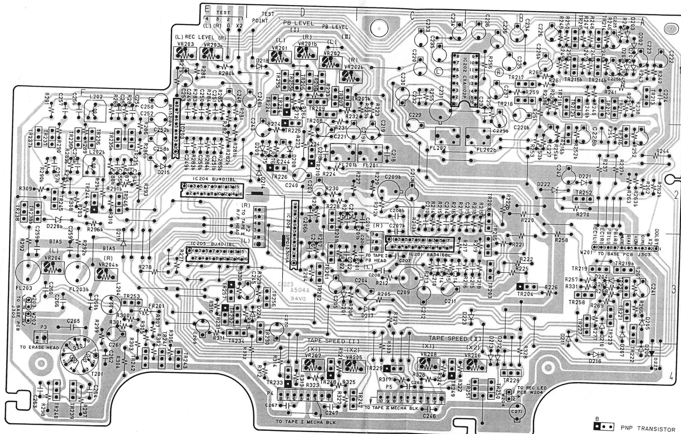
DECK PCB C1023A504A
