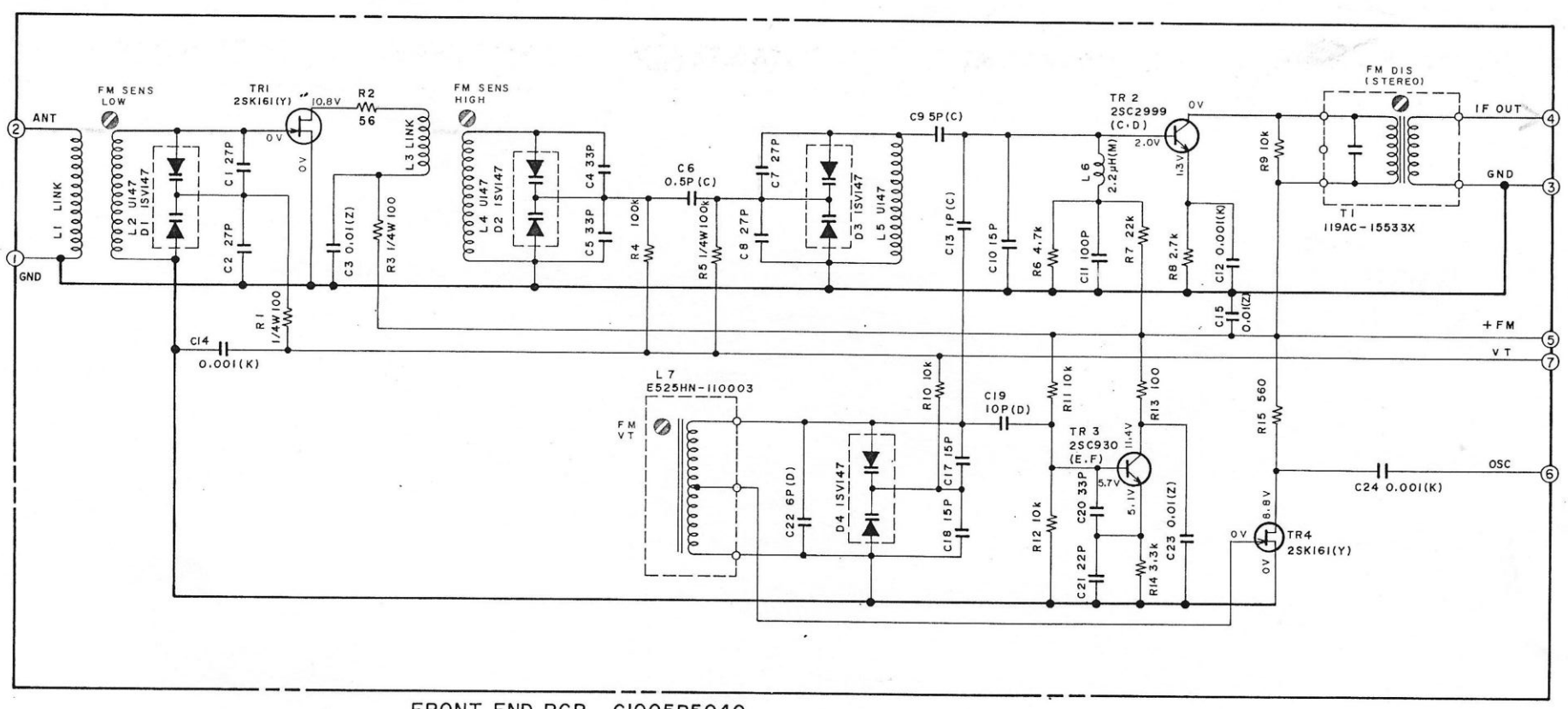
FRONT END PCB CI005B5040
