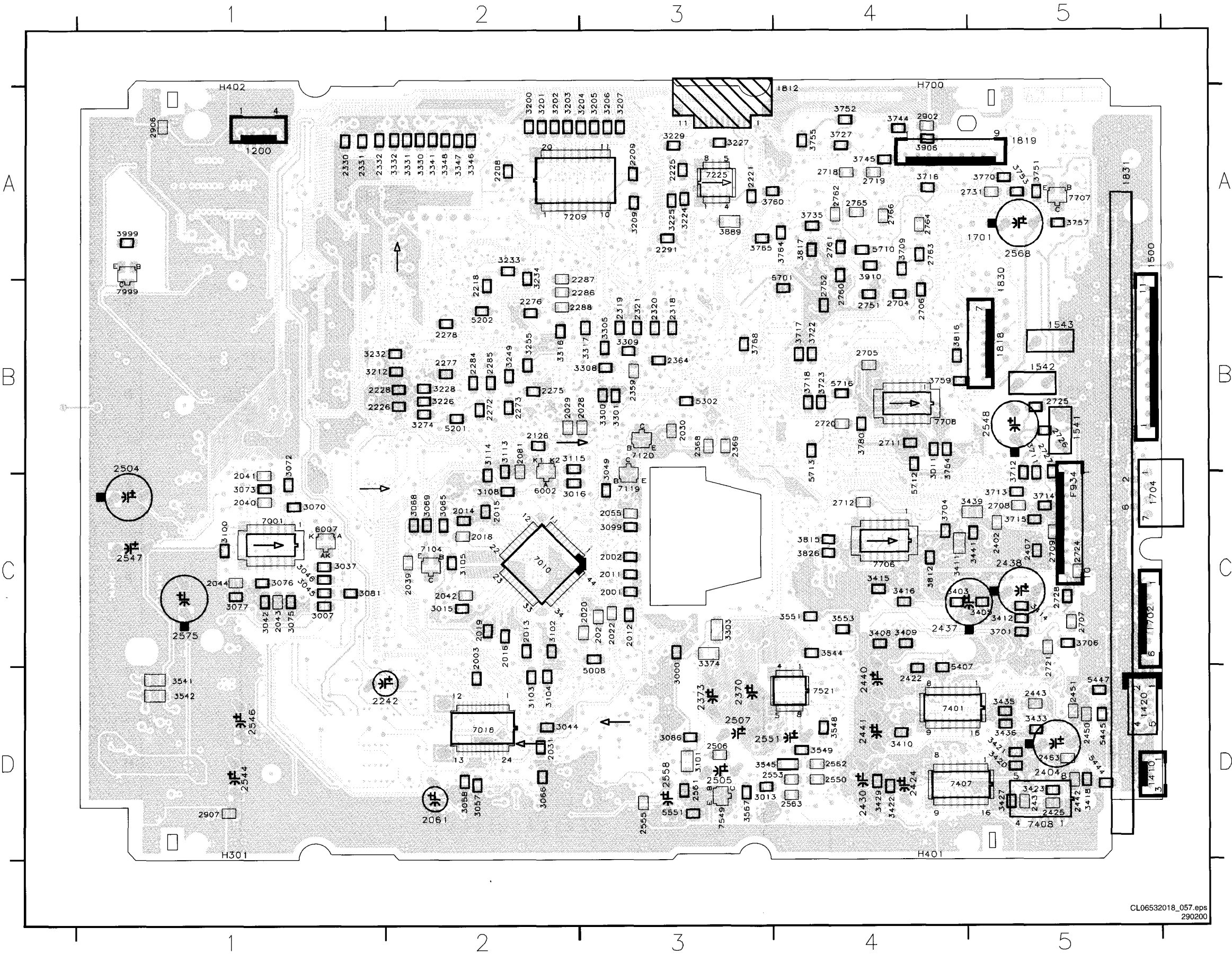
CDR MAIN BOARD .7 - BOTTOM VIEW
