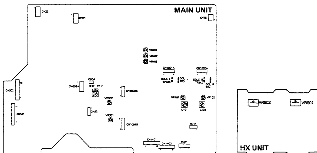
Fig. 8-2 Adjusting points
