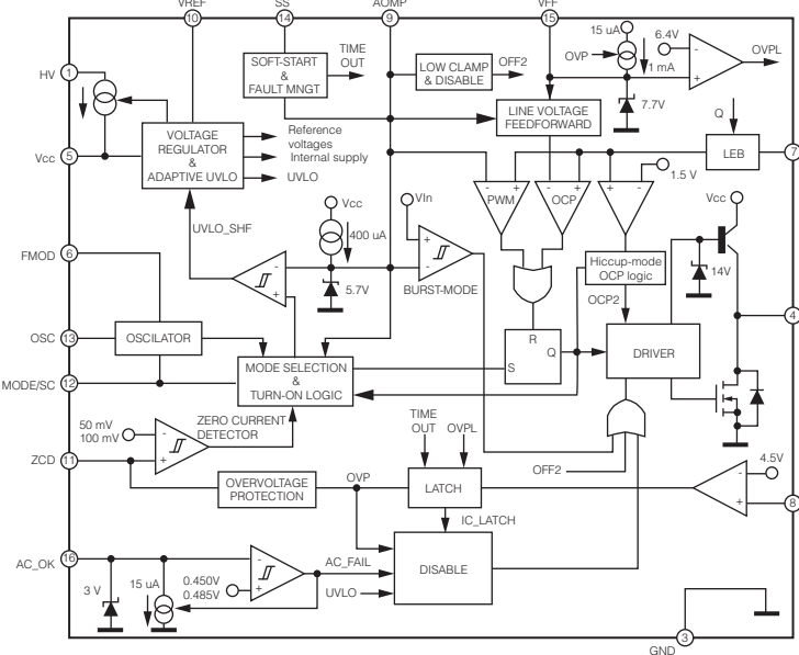
IC502: L6566BTR Multi mode controller for SMPS
