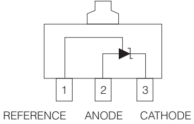
IC505: NJM431U Adjustable precision shunt regulator
