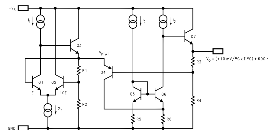
IC238: LM61CI2Z Temperature sensor
