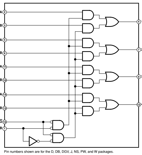
IC302, 307: SN74LV157APWR Quaduple 2-line to 1-line data selectors/multiplexers
