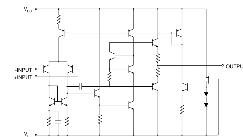
IC162-164, 169: AZ4580MTR-E1 Dual low noise operational amplifiers
