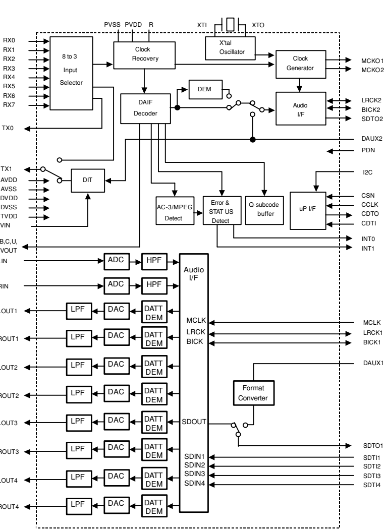
IC301: AK4588VQ 2/8-channel audio CODEC with DIR
