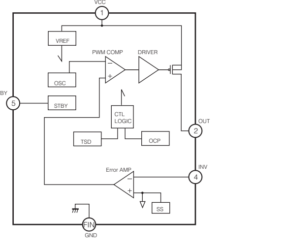
IC202: BD9870FPS-E2 High stand voltage 1 channel step-down switching regulator
