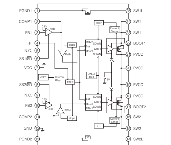
IC207: BD9302FP-E2 2.5 MHz 2 A power switch 2 ch step-down switching regulator
