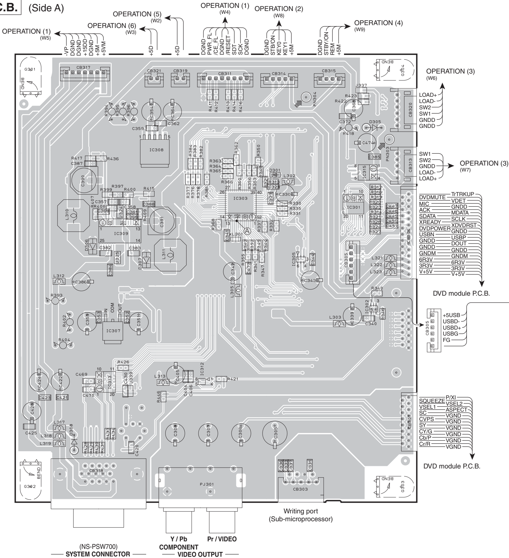
FRONT (2) P.C.B. (Side A)
