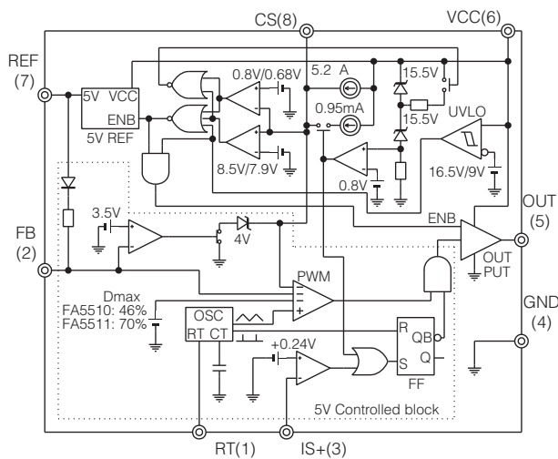
IC702: FA5511N-D1-TE1 CMOS IC for switching power supply control
