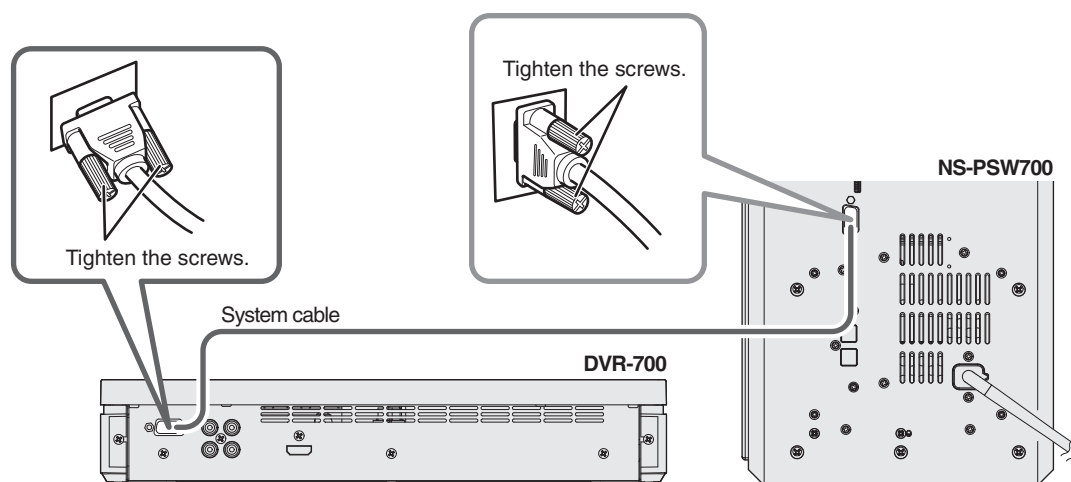
Connection Diagram 2
