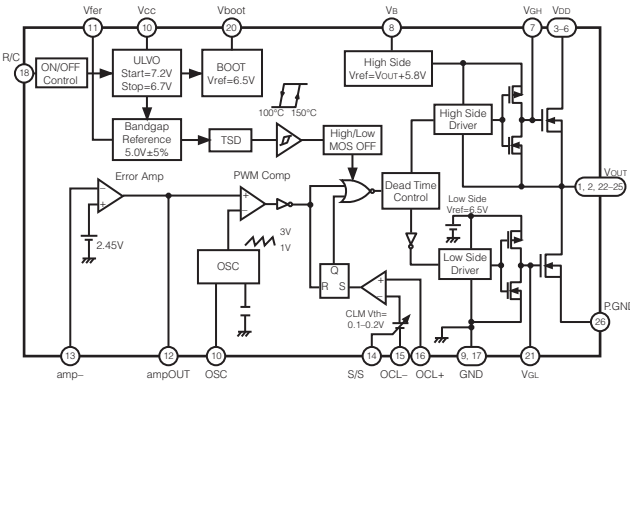
IC203: MD1423R IC power supply
