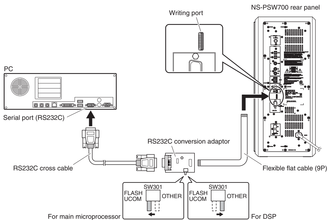
Connection Diagram 1
