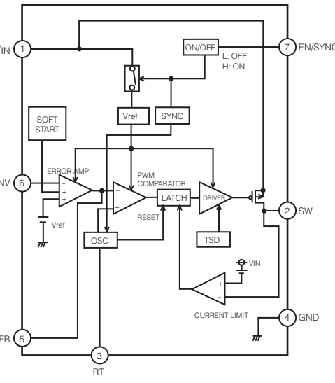
IC209: BD9781HFP Flexible step-down switching regulator
