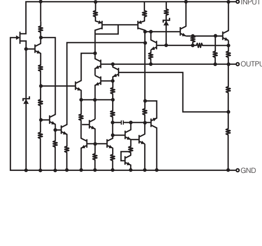
IC206: NUM7812DL1A 3 terminal voltage regulator
