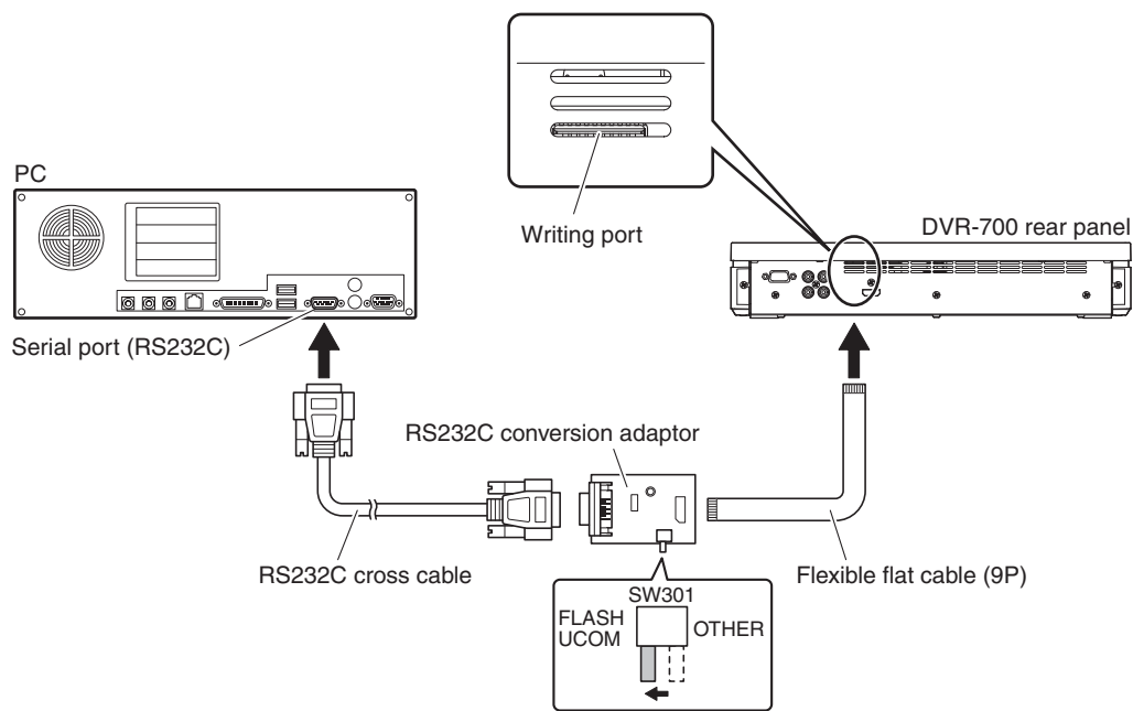
Connection Diagram 3
