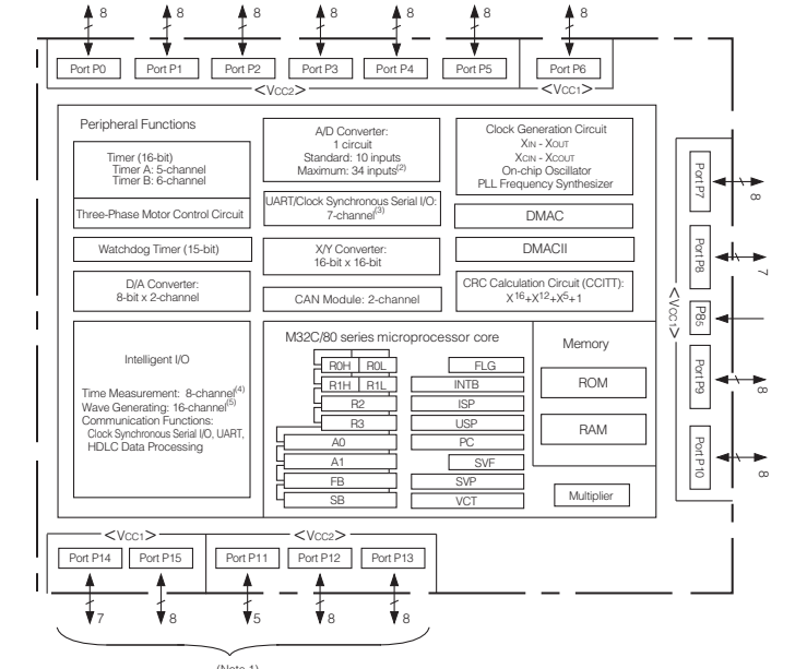
IC500: M30878JBGP Single chip 16/32-bit microprocessor
