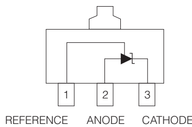
IC704: NJM431U Adjustable precision shunt regulator
